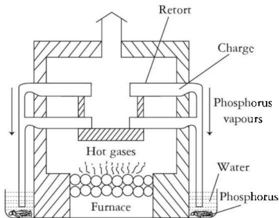
Fig 3.1 Retort process
