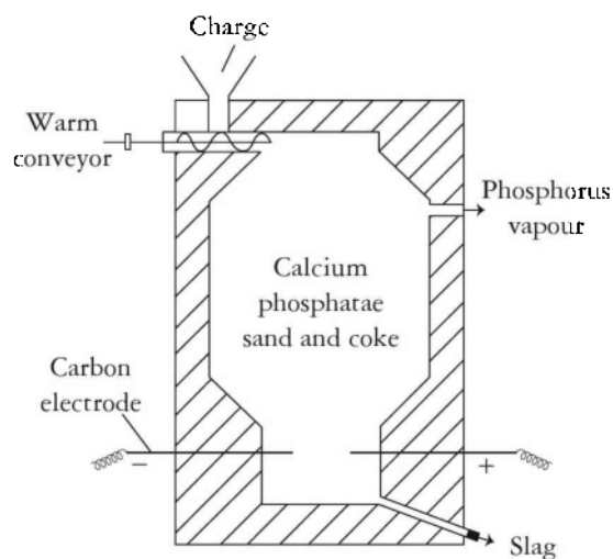
Fig 3.2 Electrothermic process
