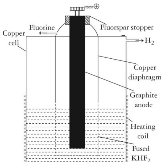
Fig. 3.4 Whytlay Method
