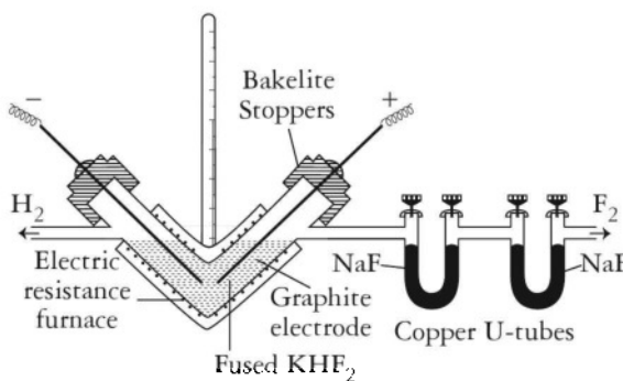
Fig. 3.3 Dennis' Method
