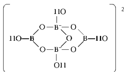
Fig. 5.5 St. of Borax
