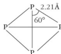
Fig. 3.9 Structure of White Phosphorous
