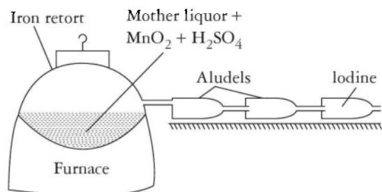
Fig. 3.6 I 2 Preparation from Kelp
