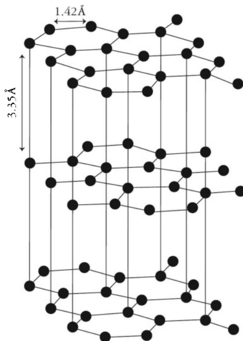
Fig 3.8. Graphite
