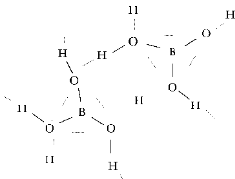
Fig. 5.4 St. of Boric acid
