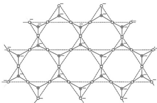
Fig. 5.11 St. of Two Dimensional Sheet Silicates
