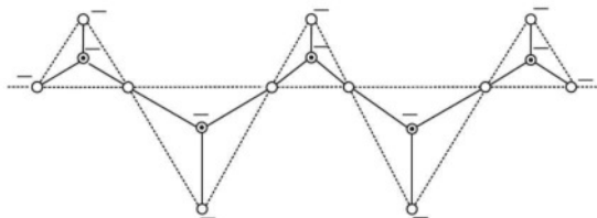
Fig. 5.10 St. of Chain Silicates
