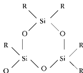
Fig. 5.7 Cyclic silicone
