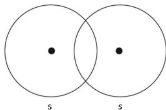
Fig. 1.3 Formation of hydrogen molecule by s-s overlapping.
