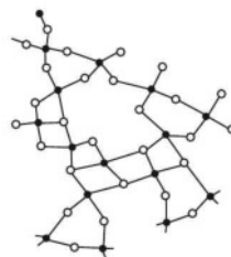
Fig. 5.12 St. of 3-dimensional Sheet Silicates
