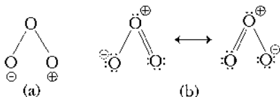
Fig. 6.3 (a) Geometry of ozone molecule (b) Resonance in ozone molecule
