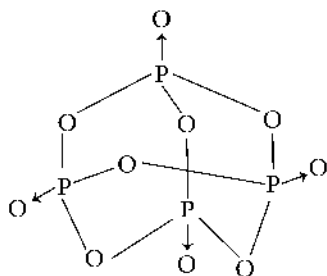
Fig. 5.17 Str. of P_4O_{10}
