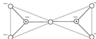
Fig. 5.8 St. of Pyrosilicates
