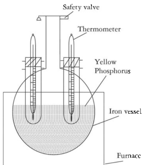
Fig. 3.10 Preparation of Red Phosphorous
