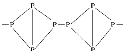
Fig. 3.11 Structure of Red Phosphorous
