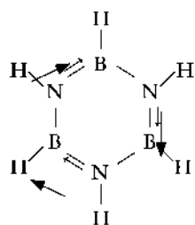
Borazine
