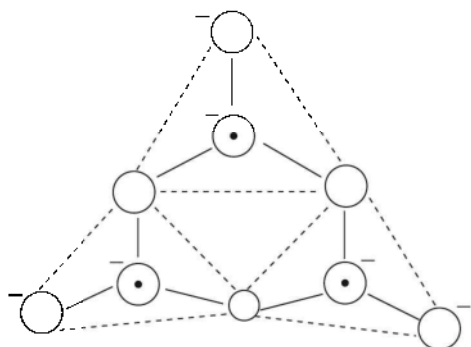
Fig. 5.9 St. of Ring Silicates
