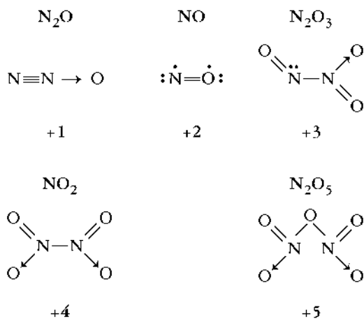
Fig 5.13 Shapes of N-oxides
