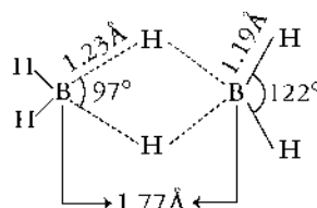
Fig. 5.2 St. of Diborane
