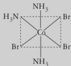
Meridional or mer-isomer
